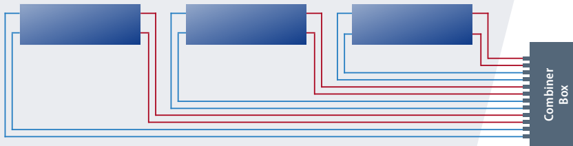
LEONI Interconnectivity DC String Cabling System
